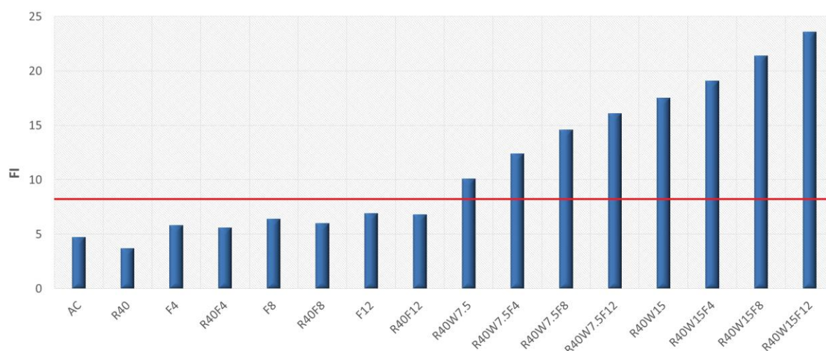
Fig. 6. IFIT results *.
