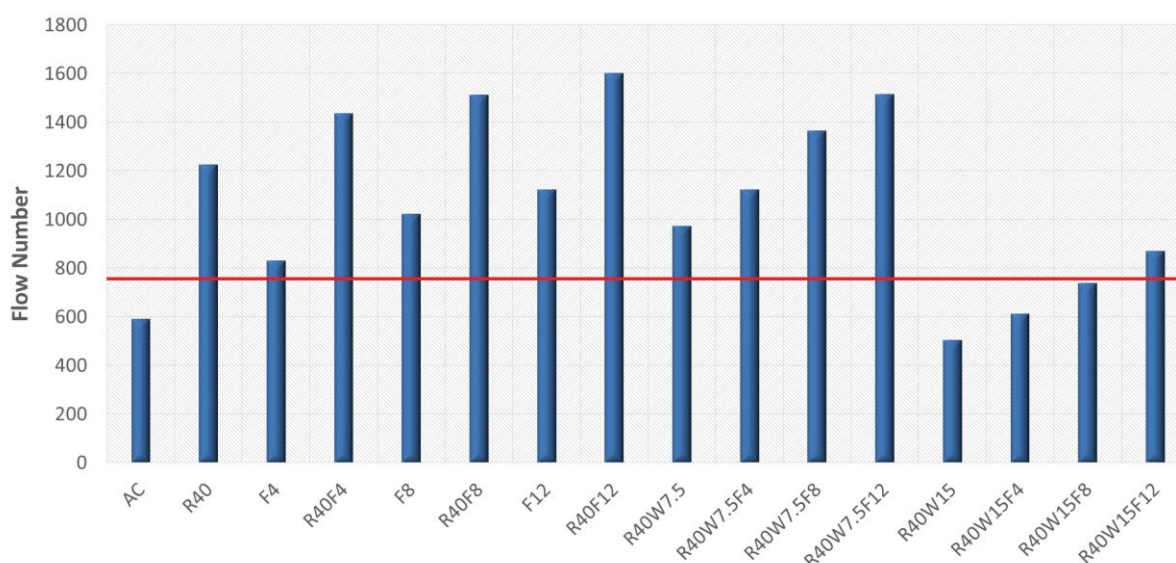
Fig. 5. Dynamic creep test results *.
