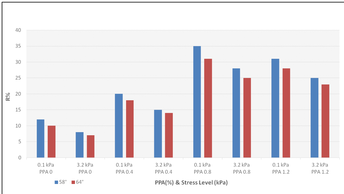
Fig. 7. Plot of R% for PPA-modified bitumen emulsion at different levels of stress and temperature.
