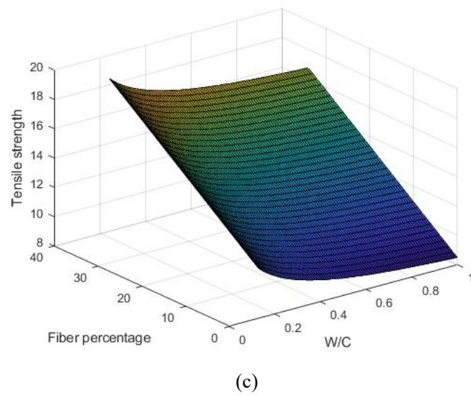
Fig. 4. Tensile strength behavior based on fiber type (a) Flat (b) Waved (c) Hooked end.
