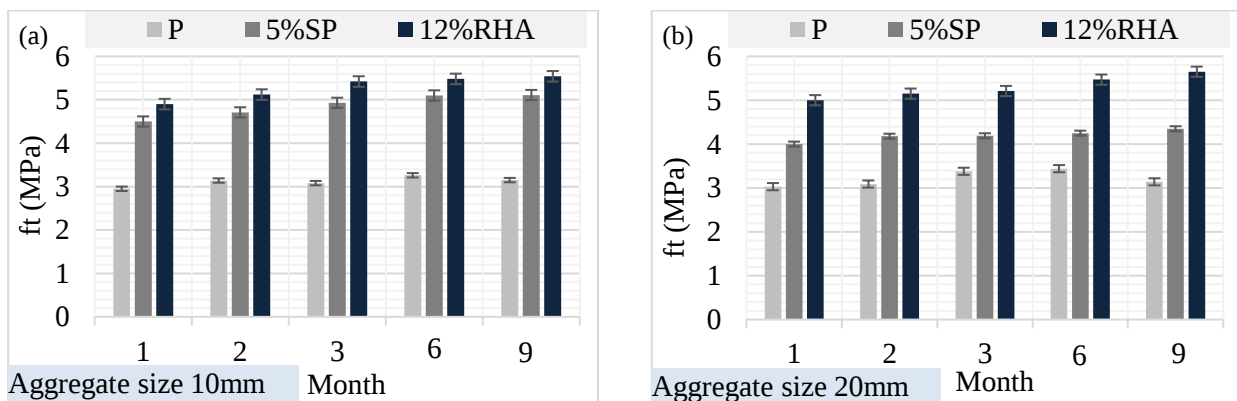
Fig. 5. Tensile splitting strength versus curing period for plain and blended concretes with: (a) 10mm; (b) 20mm maximum size of coarse aggregate.
