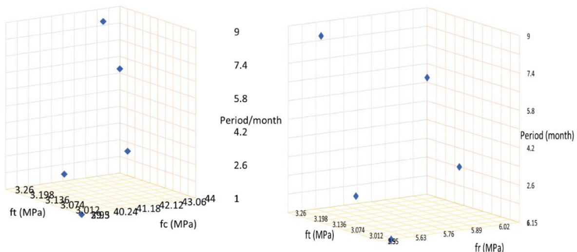
Fig. 13. Three D scatter plot: (a) f_t - f_c vs period; (b) f_t - f_r vs period for plain concrete with 10mm maximum aggregate size.
