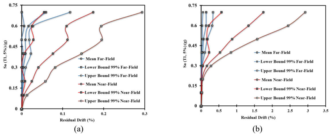
Fig. 18. Comparing 99% confidence intervals for average IDA curves of far-fault and near-fault ground motions in residual drift: (a) 8-story structure, and (b) 12-story structure.
