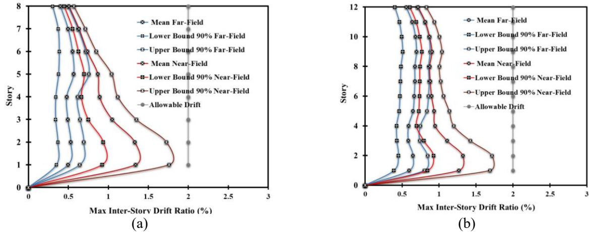
Fig. 17. Comparing 90% confidence intervals for average inter-story drift ratio of far-fault and near-fault ground motions at DBE hazard level: (a) 8-story structure, and (b) 12-story structure.
