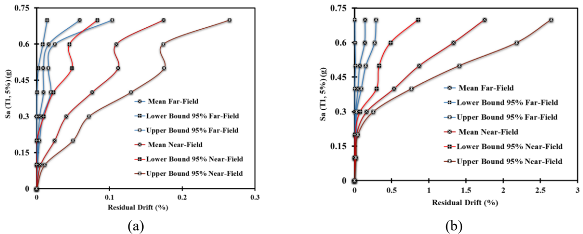
Fig. 19. Comparing 95% confidence intervals for average IDA curves of far-fault and near-fault ground motions in residual drift: (a) 8-story structure, and (b) 12-story structure.
