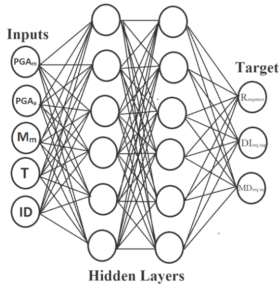
Fig. 5. Schematic view of inputs and targets.
