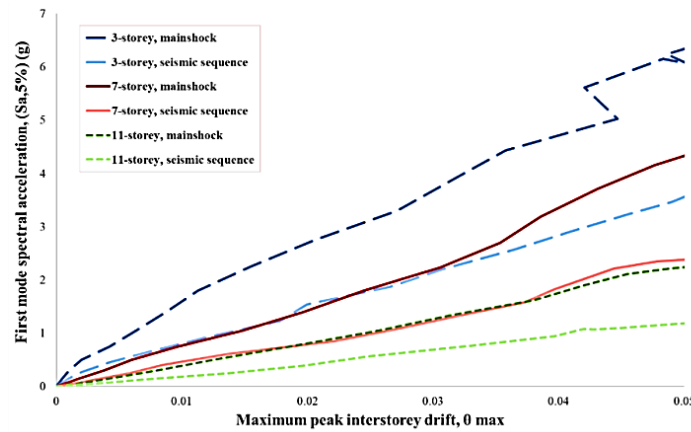
Fig. 8. Mean of IDA curves in 3, 7 and 11-story frames under single and critical successive earthquakes.
