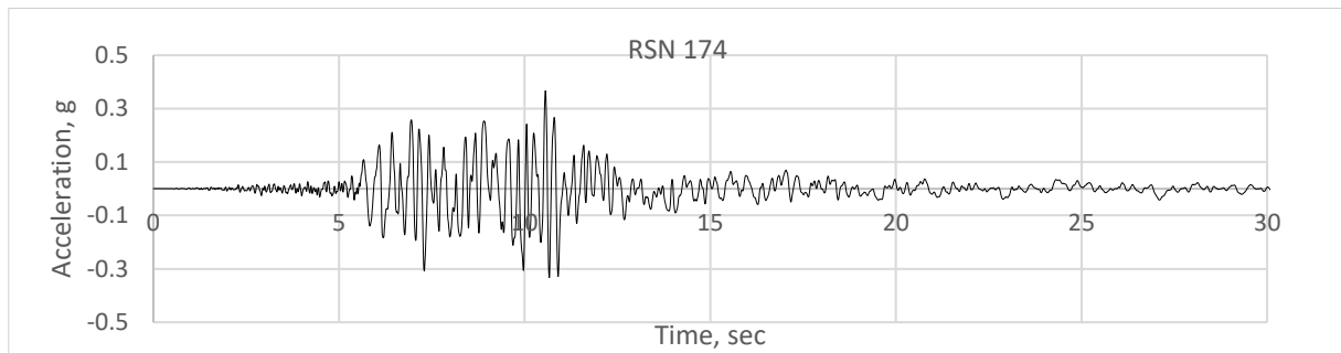
Fig. 4. RSN 174 earthquake acceleration record.
