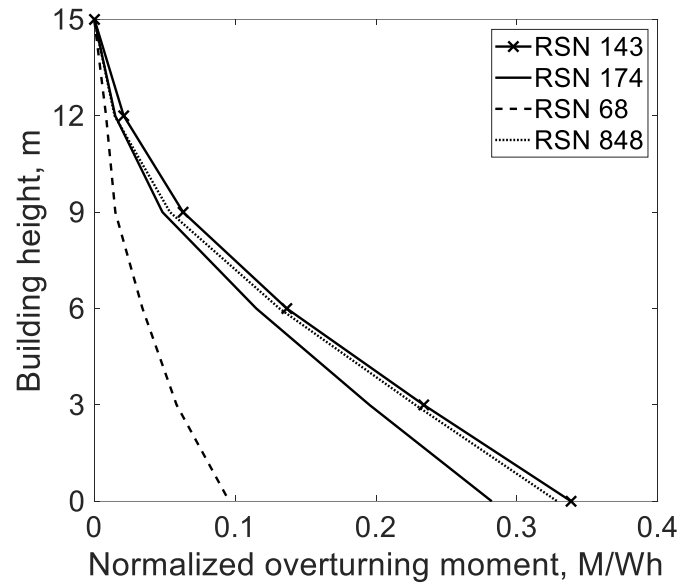
Fig. 12. Normalized overturning moment of CSB against records.
