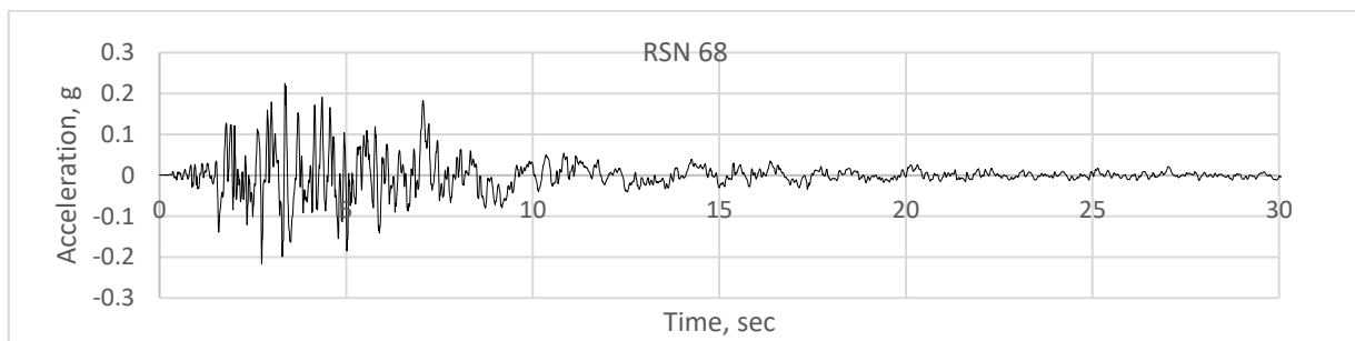
Fig. 5. RSN 68 earthquake acceleration record.
