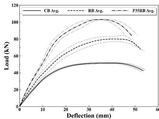
Fig. 23. Load- mid span deflection diagrams for the beams.
