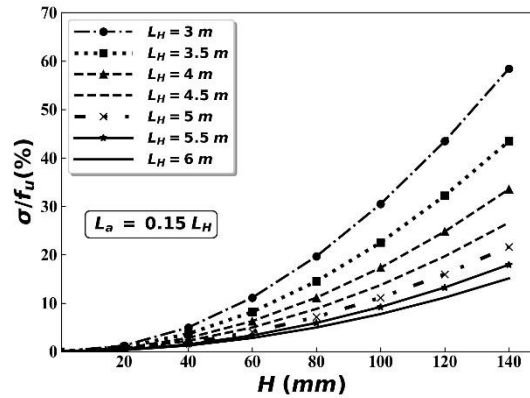
Fig. 26. The effect of L_H on the amount of FRP pre-stressing.
