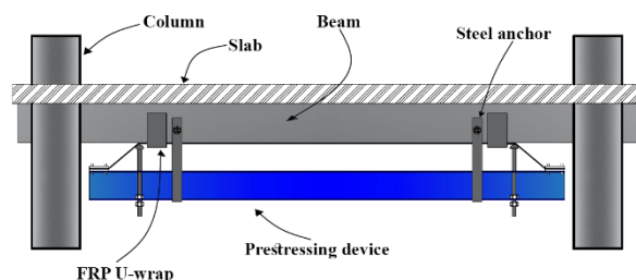
Fig. 27. Application of the FRP pre-stressing system in practice.
