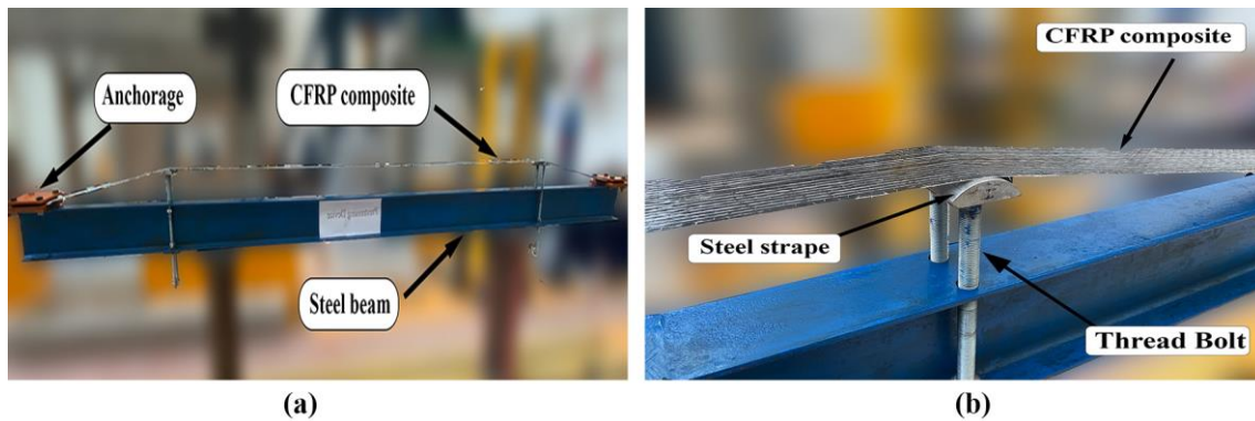
Fig. 17. CFRP pre-stressing system; a) overall view; b) view of the pre-stressing area.
