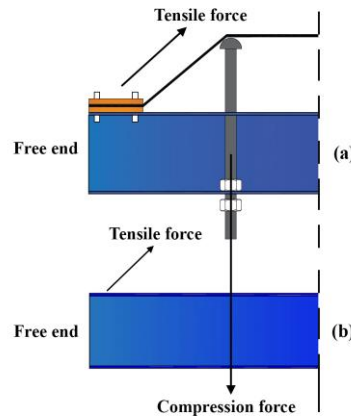
Fig. 8. Schematic view of the acting forces on the steel beam.
