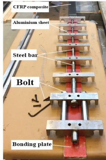
Fig. 5. Pre-stressing FRP using the method described in [25].
