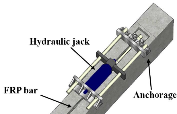
Fig. 3. Pre-stressing FRP bars.
