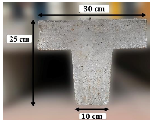
Fig. 11. Cross-section of the concrete beam.
