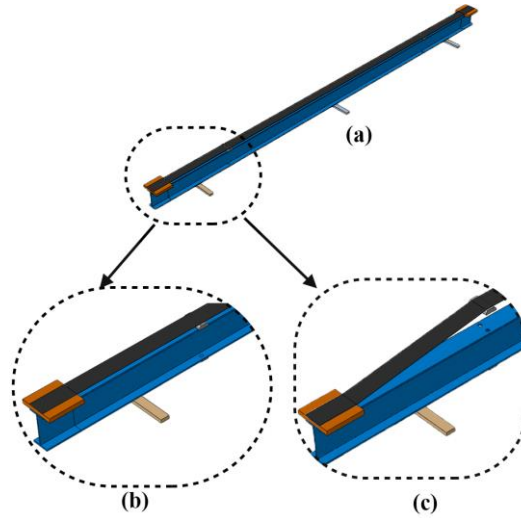
Fig. 10. Finite element model of the first part of the analysis; a) overall view; b) prior to pre-stressing; c) after pre-stressing.
