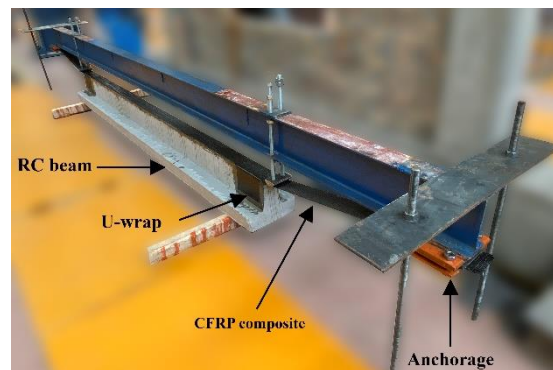
Fig. 22. Retrofitted beam using the pre-stressed CFRP.
