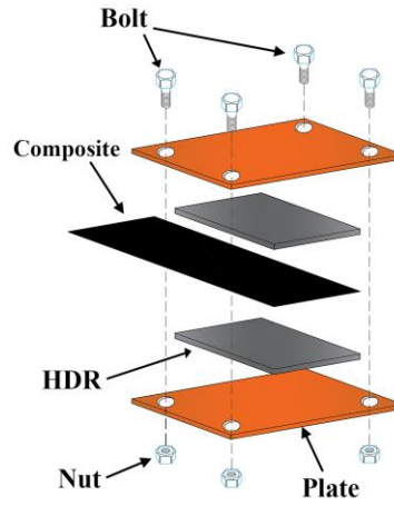
Fig. 7. The design of the anchorage area.
