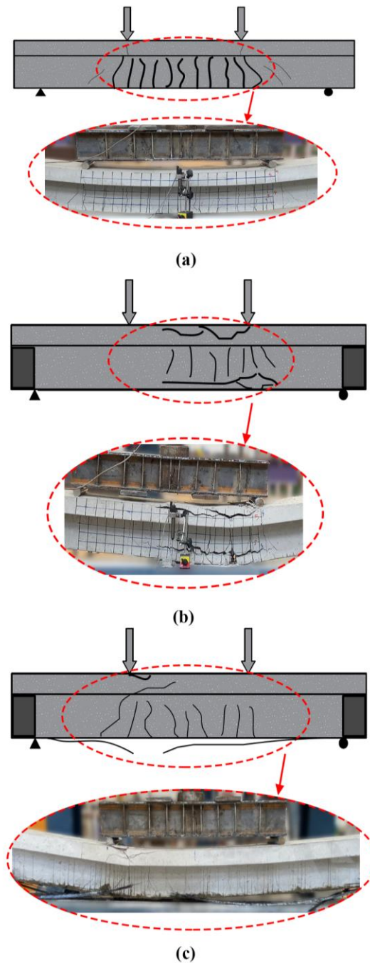
Fig. 24. Schematic view of the cracking pattern and failure modes of the beams; a) CB; b) RB; c) P35RB.
