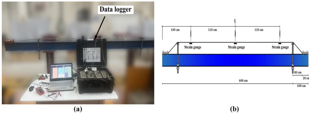
Fig. 19. Measuring the induced strain in the CFRP; a) data logging equipment; b) the location of the strain gauges.
