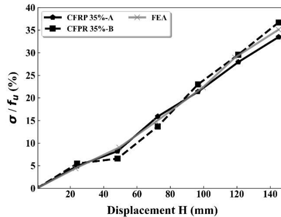
Fig. 20. Experimental and numerical results for pre-stressing the CFRP.
