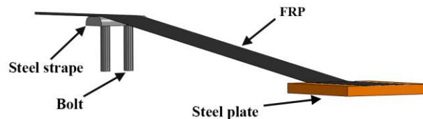
Fig. 9. Finite element model of the first part of the analysis.
