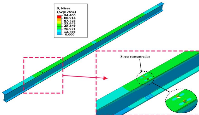
Fig. 15. Stress concentration in the steel beam (units is MPa).
