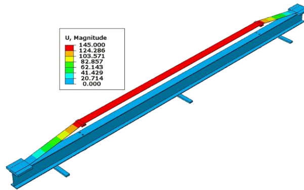
Fig. 13. Elevation induced in the CFRP for pre-stressing (units is mm).
