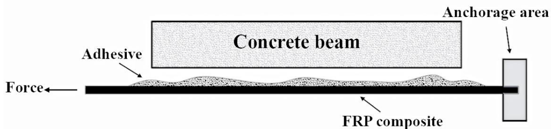
Fig. 1. FRP pre-stressing using Triantafillou et al. method [20].
