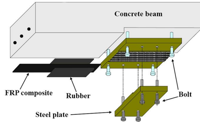
Fig. 2. Typical FRP anchorage system [13].
