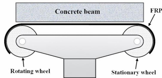
Fig. 4. Pre-stressing FRP using rotational wheels [23].
