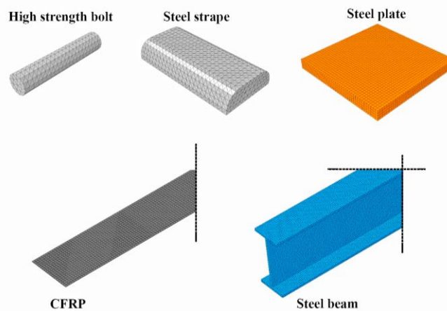
Fig. 12. Meshing of the parts of the finite element model.
