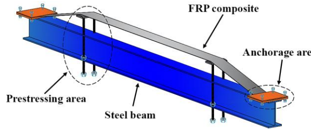
Fig. 6. The design of the innovative FRP pre-stressing system.
