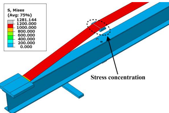
Fig. 14. Induced stress in composite (units is MPa).
