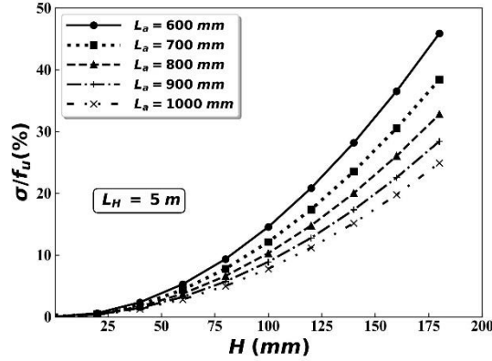
Fig. 25. The effect of L_a on the amount of FRP pre-stressing.
