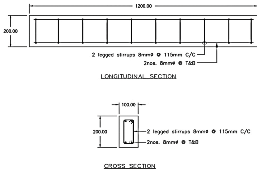
Fig. 2. Detailing of the Beam.
