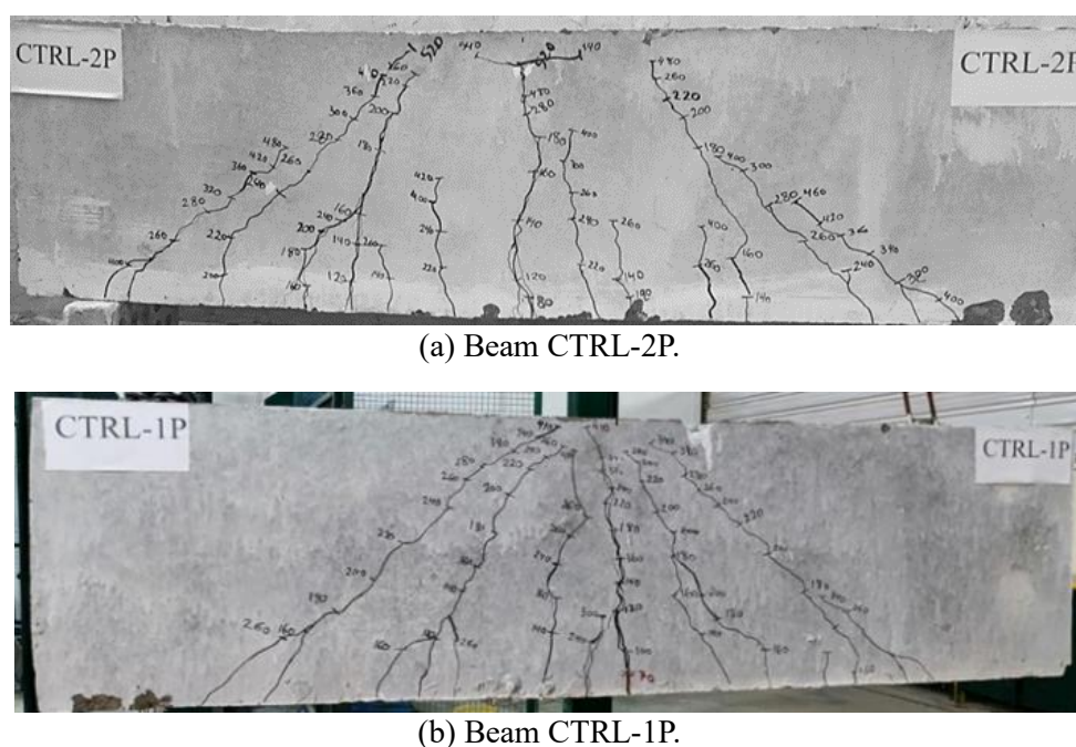
Fig. 5. Crack patterns of the control specimens.
