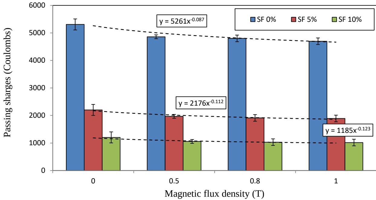
Fig. 13. Effect of applying different MF intensities on passing charges in RCP test.
