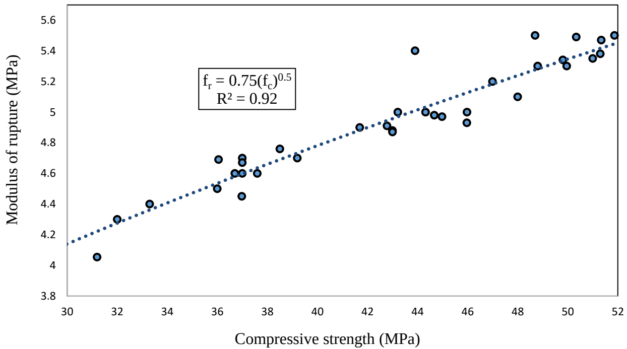
Fig. 11. Variation of mechanical strengths of concrete exposed to different MF intensities.
