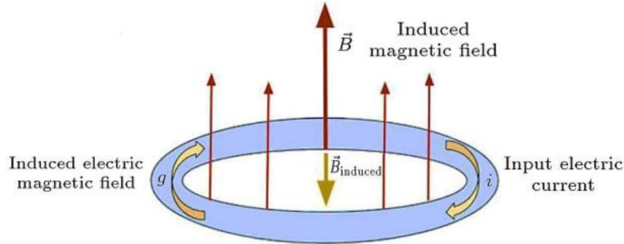
Fig. 2. The pattern of the magnetic flux lines around the current-carrying circular loop [24].
