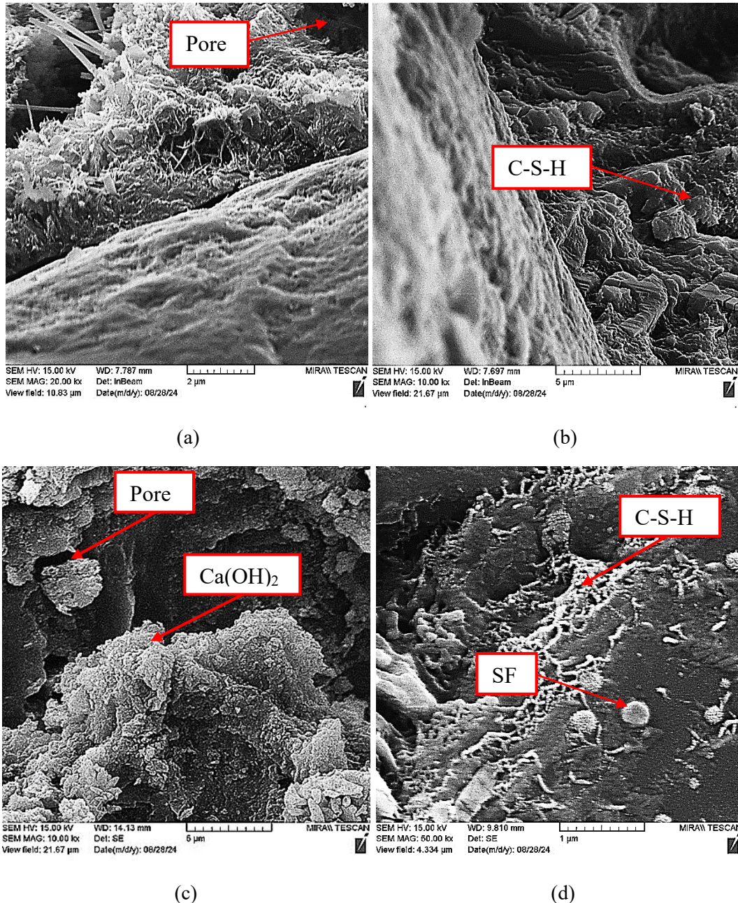
Fig. 16. Microstructure of concrete by means of SEM imaging, (a) N.Mag, (b) Mag, (c) N.Mag-SF10, (d) Mag-SF10.
