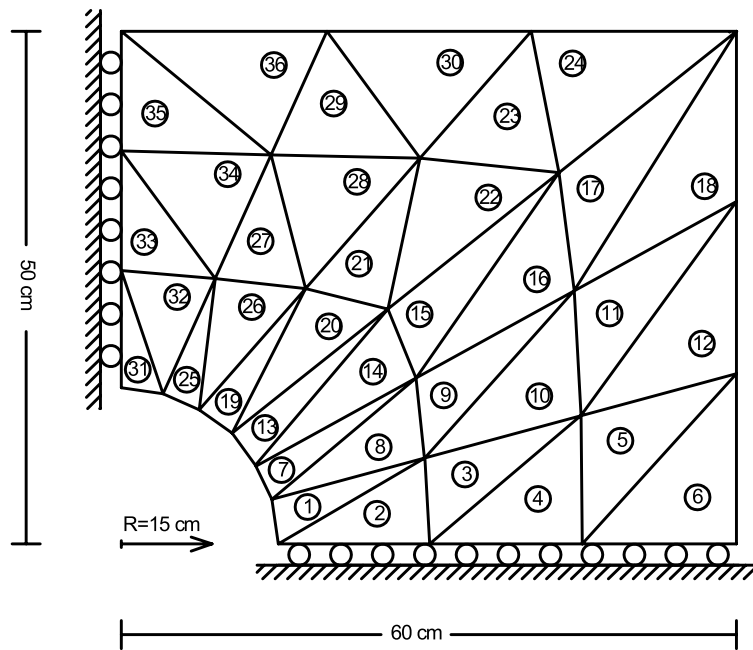
Fig. 5: Rectangular plate with a quarter-circle cutout [27].
