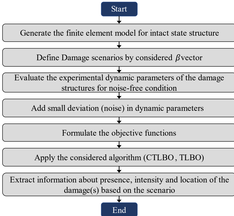
Fig. 1. Damage detection approach.
