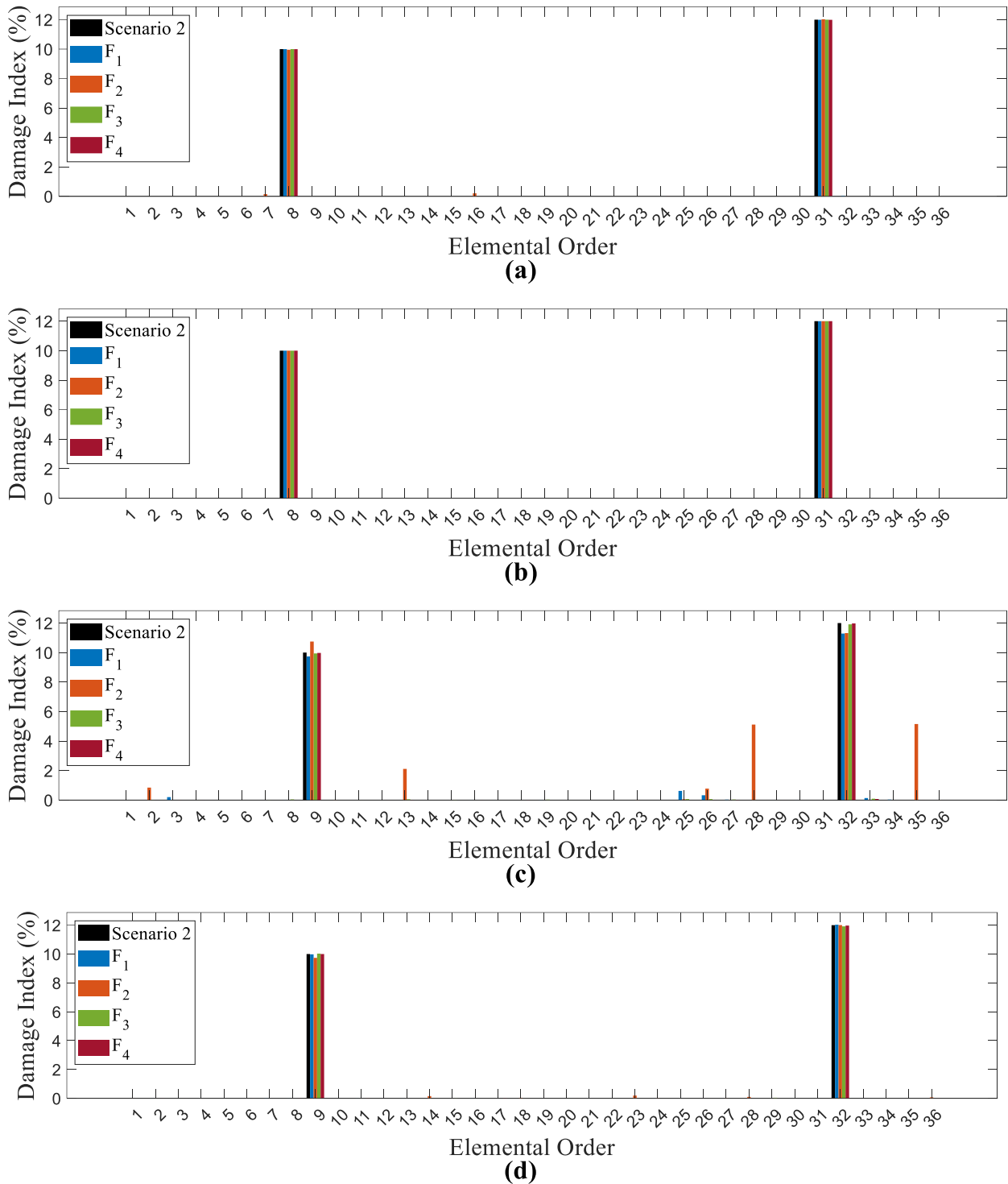
Fig. 9. Damage detection and localization of the Rectangular plate with a quarter-circle cutout for scenario 2: (a) TLBO, (b) CTLBO, (c) TLBO with noise, (d) CTLBO with noise.
