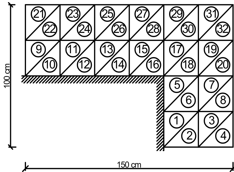
Fig. 4: An L-plate with dual clamps [27].
