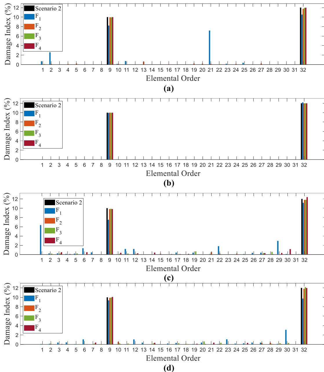
Fig. 7. damage detection and localization results of the L-plate with dual clamps for scenario 2: (a) TLBO, (b) CTLBO, (c) TLBO with noise, (d) CTLBO with noise.
