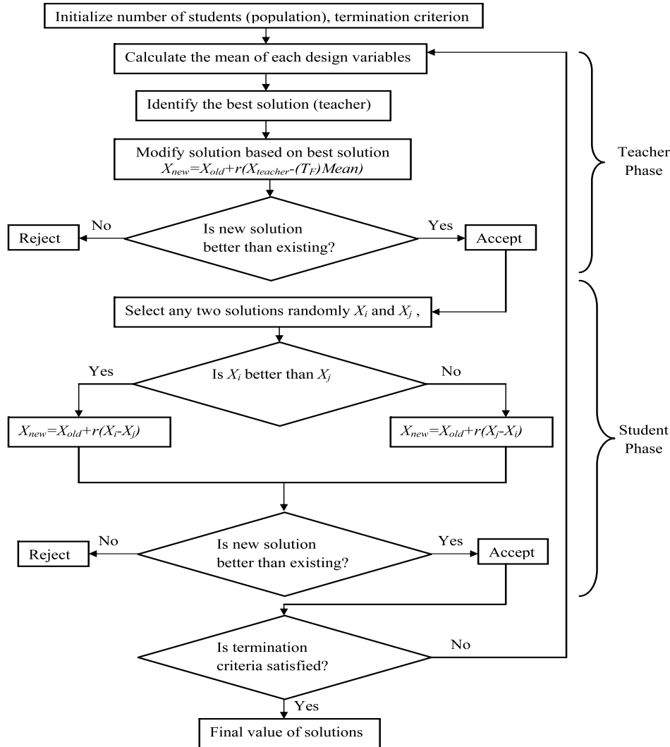
Fig. 3. Flowchart for TLBO [42].
