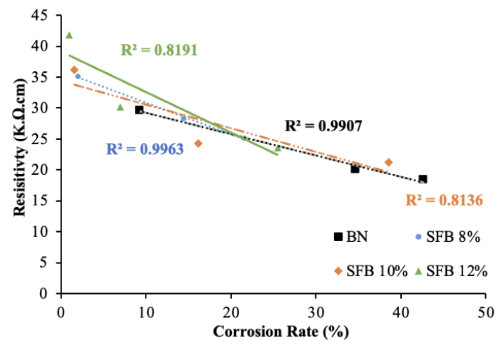
Fig. 15. Relationship between resistivity and corrosion rate with different corrosion duration.
