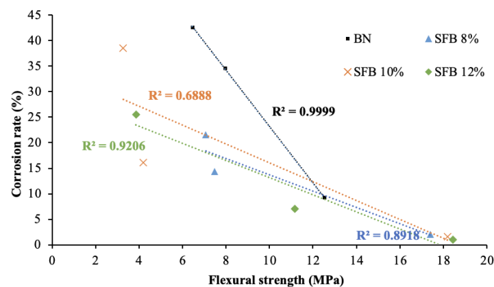
Fig. 17. Relationship between flexural strength and corrosion rate.
