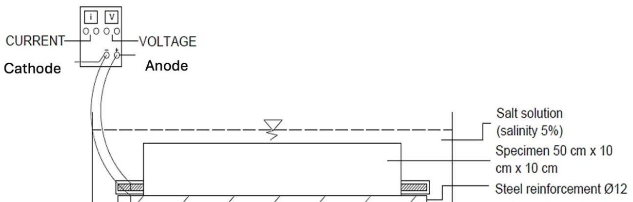
Fig. 4. Sketch of accelerated corrosion testing.
